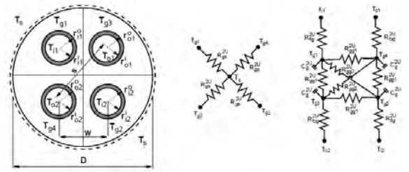
Figure 2: Inner pipe-grout heat flux resistance relationships of a 2U borehole
