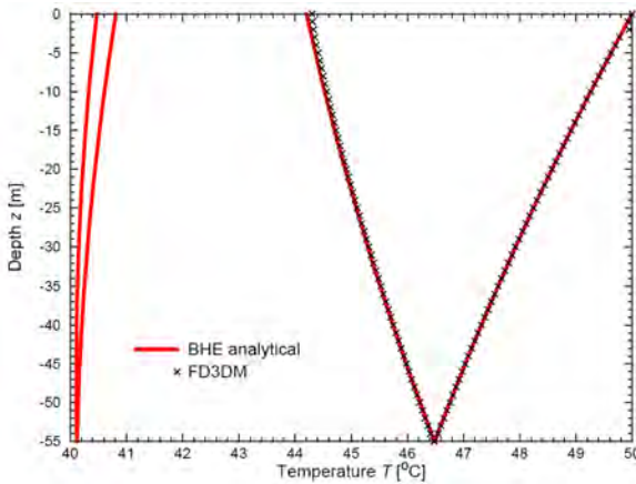
Figure 8: Analytical BHE solution of temperature profile at t = 12 hours in comparison to the fully discretized 3D model (FD3DM)
